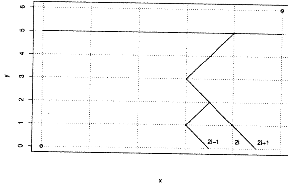
Figure 3: Path counting recursion
