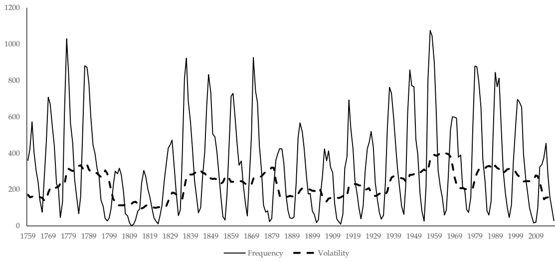
Figure 1: Frequency and volatility of sunspots from 1749 to 2017.
